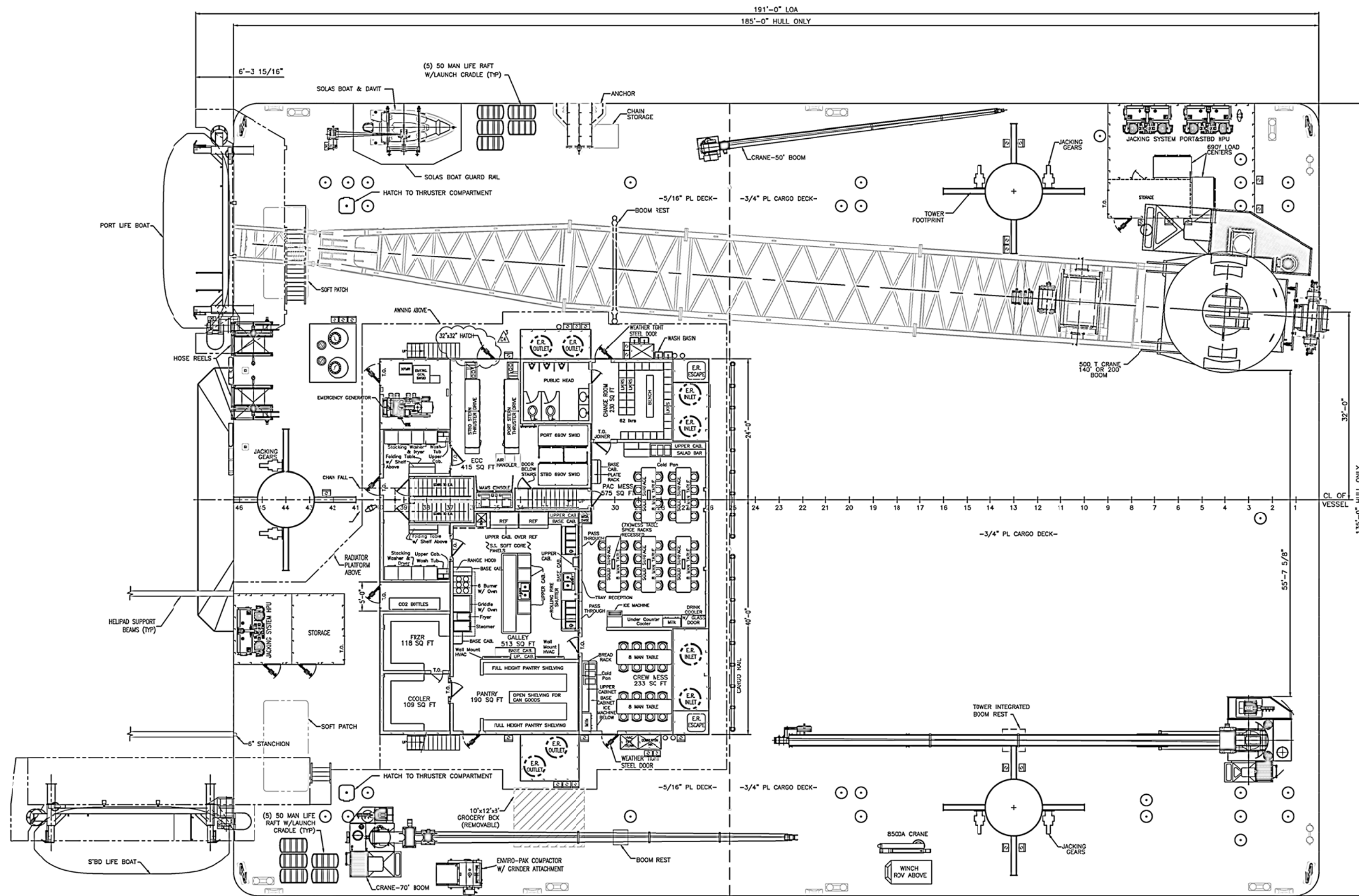
MAIN DECK PLAN
