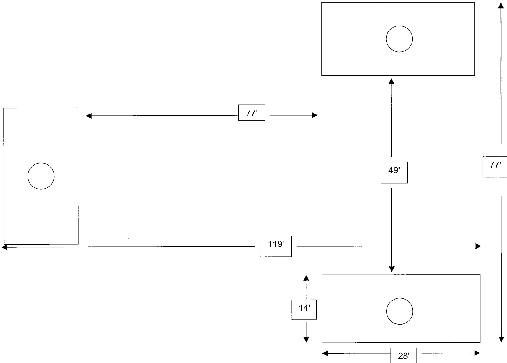
L/B Tammy (Distance between leg pads)
